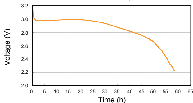
1000Ω pulse discharge at 23°C
