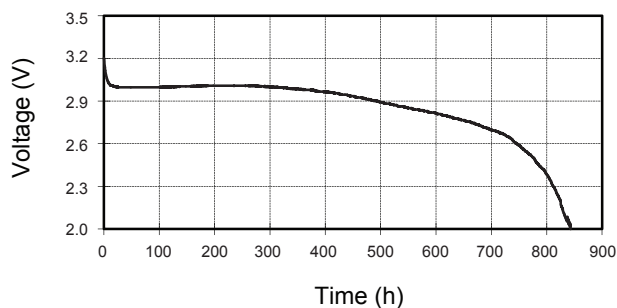
2mA continuous discharge to 2.0V at 23°C
