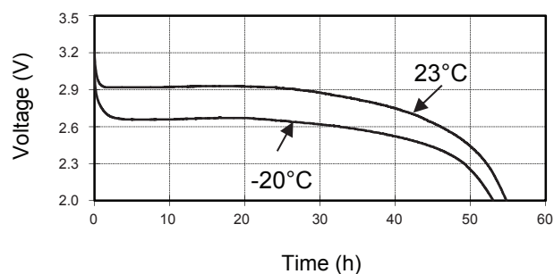
100Ω continuous discharge to 2.0V at 23°C & -20°C
