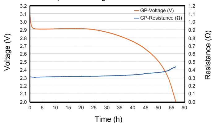
100Ω pulse discharge resistance at 23°C
